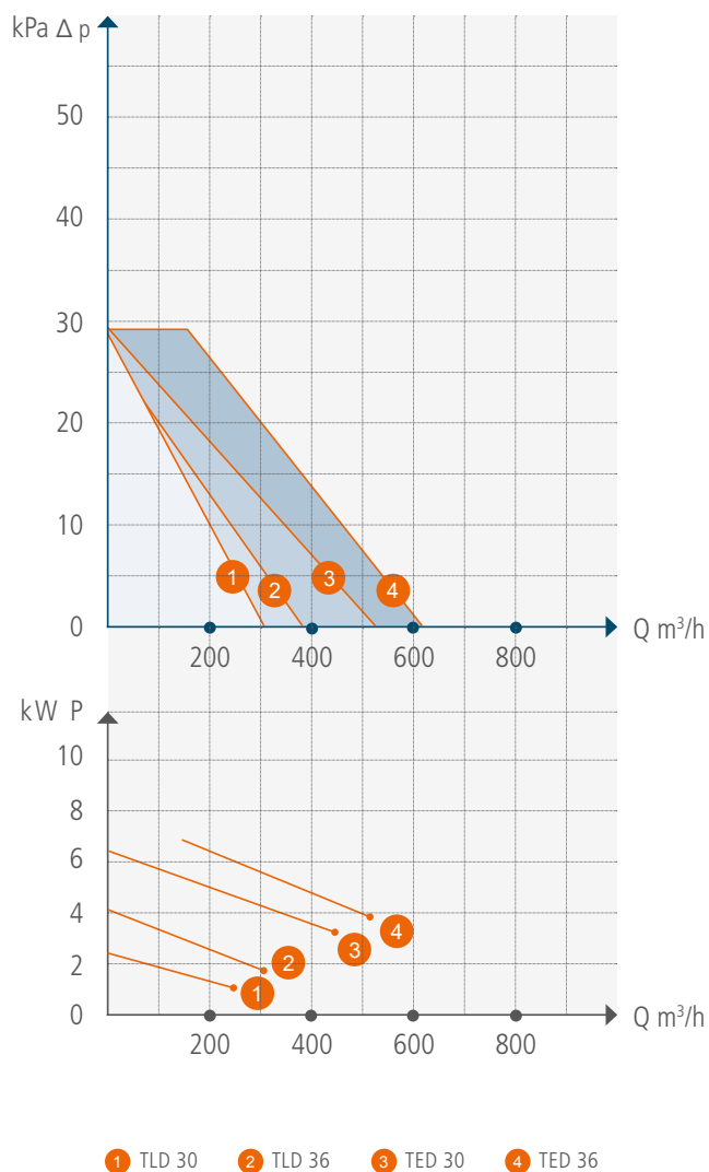
Turbopumps TLD/TED
